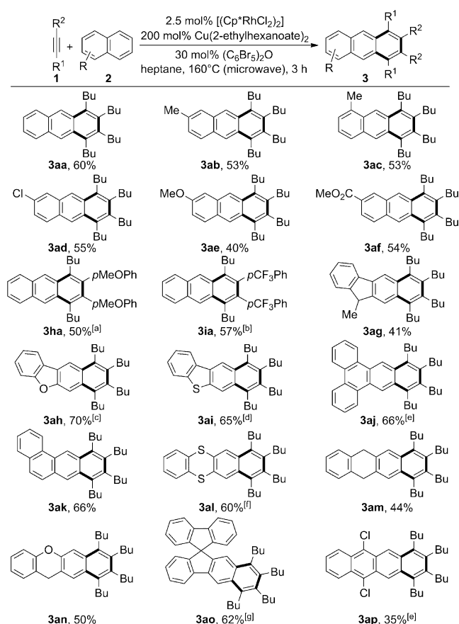
Scheme 3. Scope of the annulation process for polycyclic arenes. Reaction conditions: 1 (0.20 mmol), arene 2 (0.50 mmol), [(Cp*RhCl 2 ) 2 ] (2.50 μmol), Cu(2-ethylhexanoate) 2 (0.20 mmol), (C 6 Br 5 ) 2 O (0.03 mmol), 1.00 M in heptane, 160°C microwave heating for 3 h; All yields shown are of isolated 3 . [a] Aryl groups are 23:8:1 2,3-/2,4-/1,4-. [b] Aryl groups are 30:10:1 2,3-/2,4-/1,4-. [c] 2:1 linear/angular isomer. [d] 3.7:1 linear/angular isomer. [e] 0.50 M in heptane. [f] 3:1 linear/angular isomer. [g] reaction performed with 5.00 μmol [(Cp*RhCl 2 ) 2 ] in heptane 0.50 M for 6 h.
